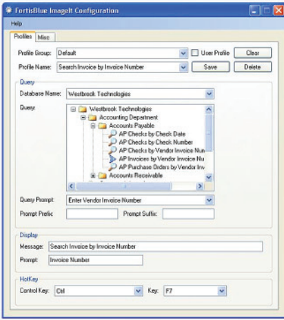
FortisBlue Imagent's intuitive administrative interface
